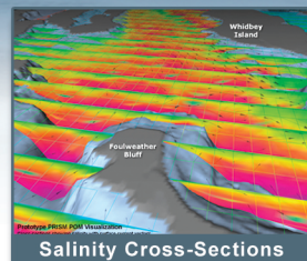
Salinity Cross-Sections
